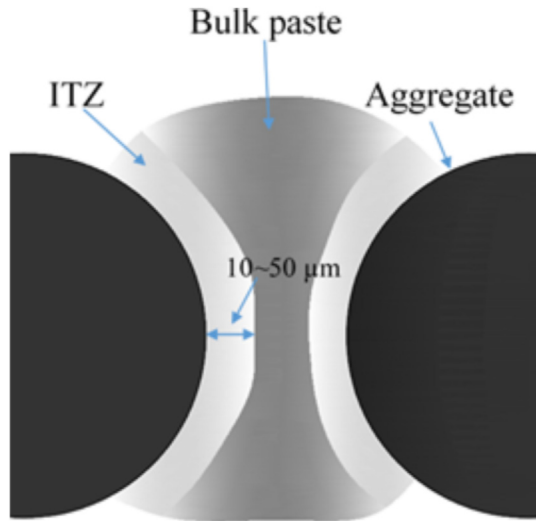
Fig. 2. Schematic diagram of the three-phase composite sphere for concrete.
