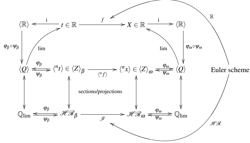
Figure 1: The skeleton of the arithmetization scheme described in [5] which links the Euclidean function f with a sequence of integer functions \langle^n f \rangle . Basically, the integer function \langle^n f \rangle is the arithmetized expression at the scale n of the Euclidean function f . The sequence \langle^n f \rangle itself is obtained as a section of the function \mathcal{F} which translate f when \mathbb{R} is replaced by the Harthong–Reeb line. The function \mathcal{F} is computed using a nonstandard version of the Euler scheme for solving differential equations.
