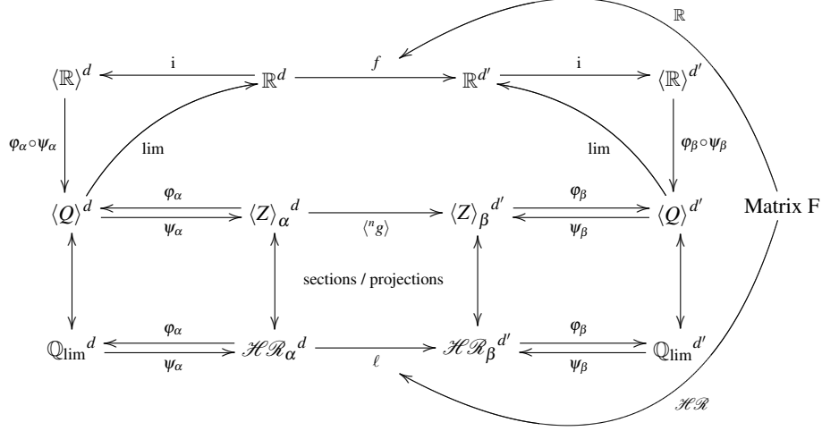
Figure 3: The \Omega -arithmetization scheme which associates to the linear transformation f the sequence of quasi-affine transformations \langle {}^n g \rangle from \langle \mathbb{Z} \rangle_\alpha^d to \langle \mathbb{Z} \rangle_\beta^{d'} . This sequence is obtained as a section of a translation of the matrix F of f using Harthong-Reeb coefficients.
