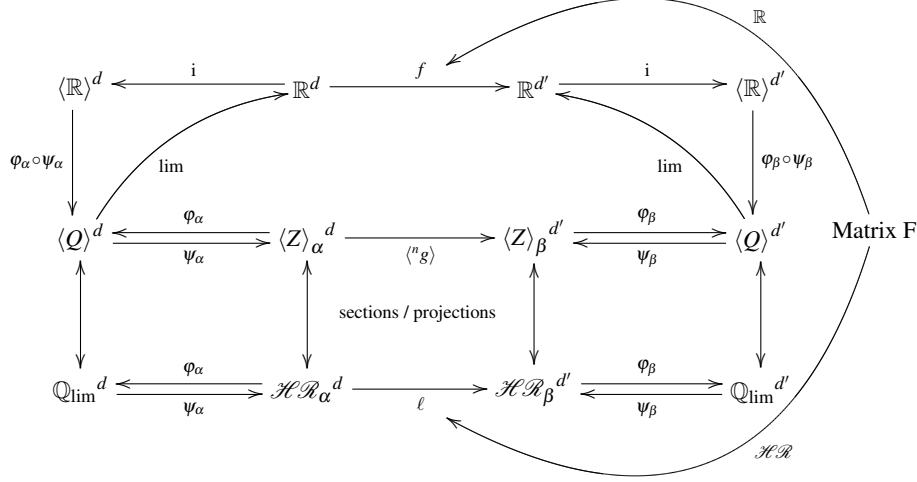
Figure 3: The \Omega -arithmeticization scheme which associates to the linear transformation f the sequence of quasi-affine transformations {}^n g from \langle \mathbb{Z} \rangle_\alpha^d to \langle \mathbb{Z} \rangle_\beta^{d'} . This sequence is obtained as a section of a translation of the matrix F of f using Harthong–Reeb coefficients.
