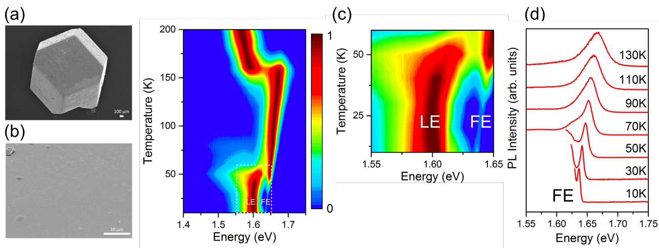
Figure 1: (a) Top view SEM image of a mm-sized \text{CH}_3\text{NH}_3\text{PbI}_3 crystal. (b) Higher resolution SEM image of the surface of the crystal. (c) PL map as a function of temperature of a single \text{CH}_3\text{NH}_3\text{PbI}_3 crystal with an enlarged view of the FE and LE band below 60K (d) Few PL spectra at different temperatures with a zoom on the FE emission.
