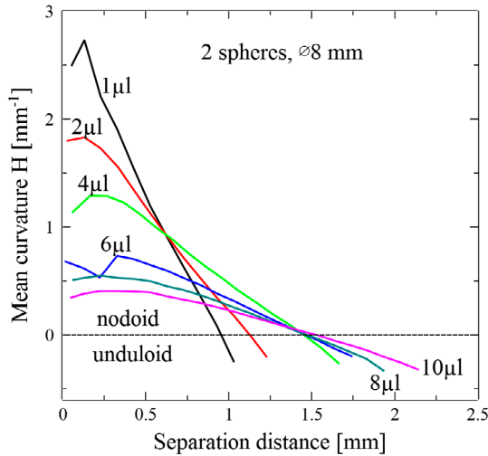
Figure 5. Mean curvature H of capillary bridge in function of interparticle distance D for the sphere of 8 mm diameter. H > 0 corresponds to the nodoid case and H < 0 to the unduloid one.
