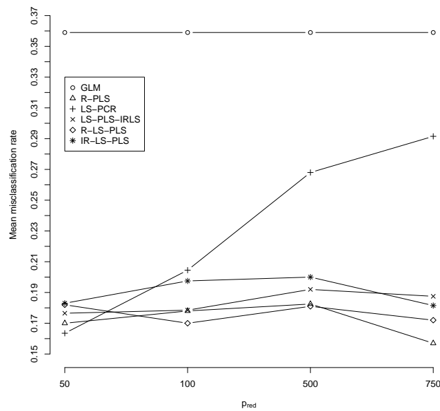
Figure 5: Evolution of mean misclassification rate from Central Nervous System data set using the six methods considering different number of relevant genes : p_{red} = 50, 100, 500 and 750 . GLM and R-PLS denote the misclassification rate and AUC obtained from GLM applied on clinical data alone and PLS to gene expression alone, respectively. LS-PCR denotes the approach derived to PCR where gene expression data are analysed using PCA and IRLS can thus applied on the merge data set of PCA-scores and clinical data. LS-PLS-IRLS, R-LS-PLS-IR-LS-PLS denote the misclassification rate and AUC obtained from the new proposed LS-PLS approaches combining expression and clinical data. For each method, a line is drawn to connect symbols to improve readability.
