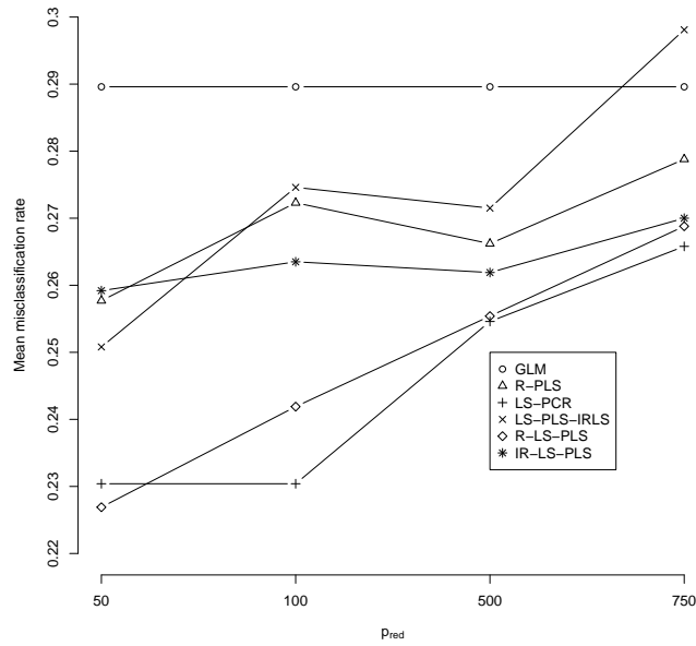
Figure 3: Evolution of mean misclassification rate from Breast Cancer data set using the six methods considering different number of relevant genes : p_{red} = 50, 100, 500 and 750 . GLM and R-PLS denote the misclassification rate and AUC obtained from GLM applied on clinical data alone and PLS to gene expression alone, respectively. LS-PCR denotes the approach derived to PCR where gene expression data are analysed using PCA and IRLS can thus applied on the merge data set of PCA-scores and clinical data. LS-PLS-IRLS, R-LS-PLS, IR-LS-PLS denote the misclassification rate and AUC obtained from the new proposed LS-PLS approaches combining expression and clinical data. For each method, a line is drawn to connect symbols to improve readability.
