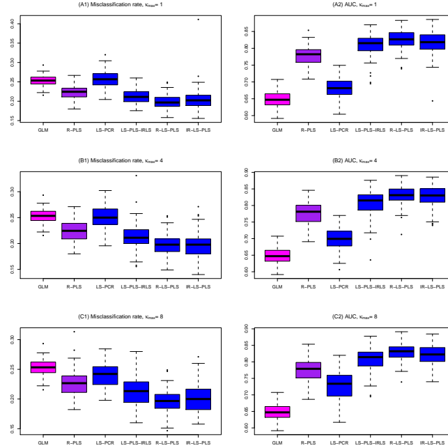
Figure 1: Boxplot of the misclassification rate (left part) and AUC (right part) from the 100 simulated data sets using the six methods, according to different \kappa_{max} : (A1, A2) \kappa_{max} = 1 ; (B1, B2) \kappa_{max} = 4 ; (C1, C2) \kappa_{max} = 8 . GLM and R-PLS denote the misclassification rate and AUC obtained from GLM applied on clinical data alone and PLS to gene expression alone, respectively. LS-PCR denotes the approach derived to PCR where gene expression data are analysed using PCA and IRLS can thus applied on the merge data set of PCA-scores and clinical data. LS-PLS-IRLS, R-LS-PLS-IR-LS-PLS denote the misclassification rate and AUC obtained from the new proposed LS-PLS approaches combining expression and clinical data . For clarity of the figure, we use a code color to indicate the predictions : from clinical data alone in pink, from expression gene data alone in purple and the results from methods combining both type of variables in blue. From SIS procedure, the relevant gene expression variables p_{red} is set to 500.
