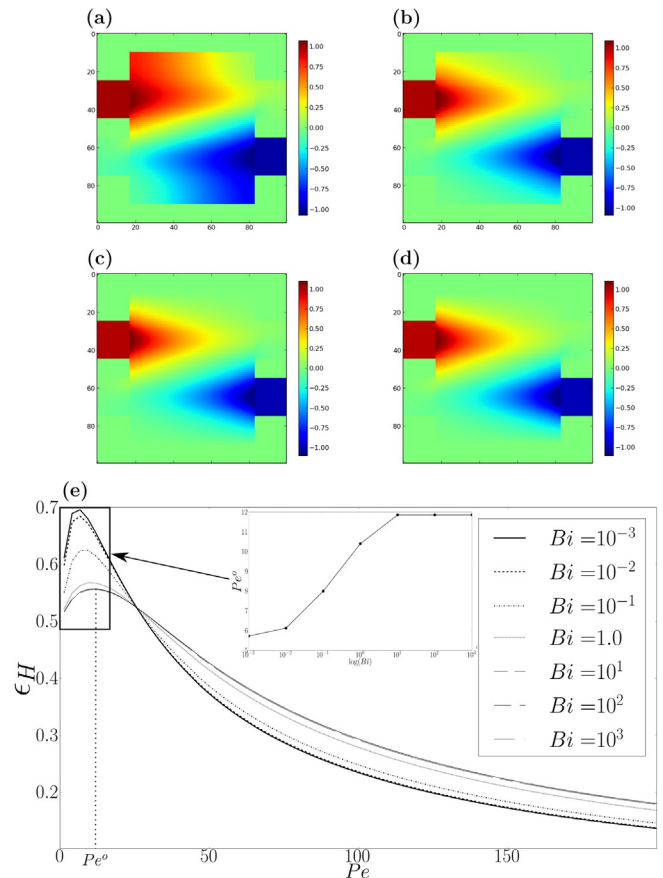
Fig. 6. Longitudinal temperature fields at Pe = 25 , L^* = 20 , \frac{k^S}{k^F} = 1 for (a) Bi = 10^{-3} , (b) Bi = 1 , (c) Bi = 10 , (d) Bi = 10^3 . (e) \epsilon_H against Péclet for L^* = 20 and Bi = 10^{-3}, 10^{-2}, 10^{-1}, 1, 10^1, 10^2, 10^3 . Inset figure is Péclet at maximum hot effectiveness against \log(Bi) .
