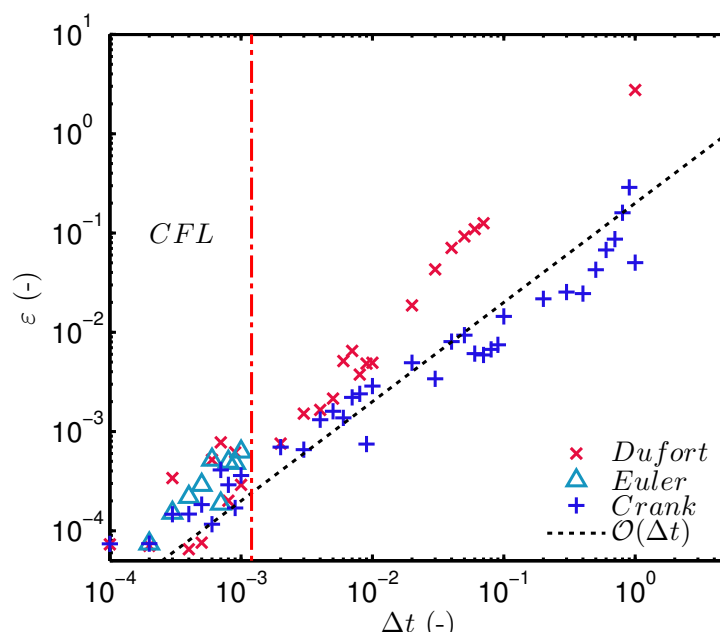
Figure 10. \mathcal{L}_2 error (a) as a function of \Delta t .
