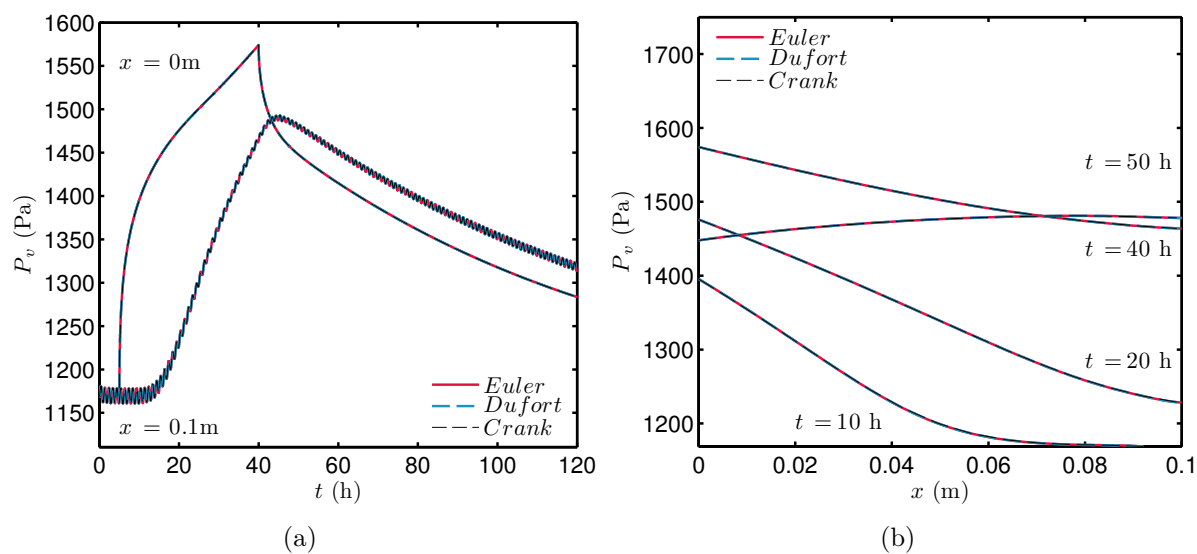
Figure 8. Vapour pressure time evolution at x \in \{0, 0.1\} m (a) and profiles for t \in \{10, 20, 40, 50\} h (b).
