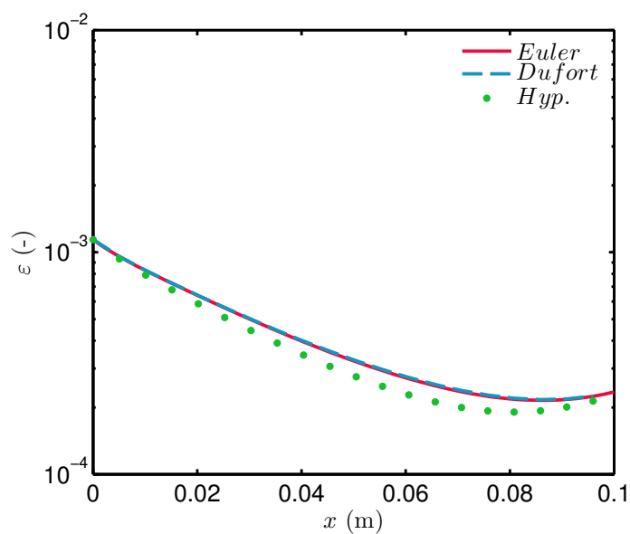
Figure 4. L_2 error for fixed \Delta t = 10^{-4} .
