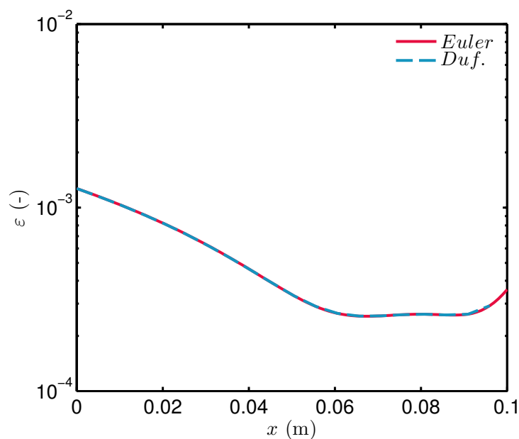
Figure 9. L_2 error for a fixed \Delta t = 6 \cdot 10^{-6} .
