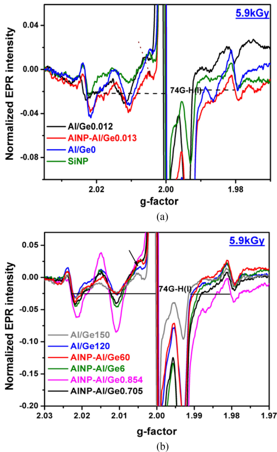
Fig. 3. EPR spectra of \text{Er}^{3+} doped germano-silica fibers at 1 mW, 3.0 G (a) low content of Al/Ge ratio and (b) high content of Al/Ge ratio.
