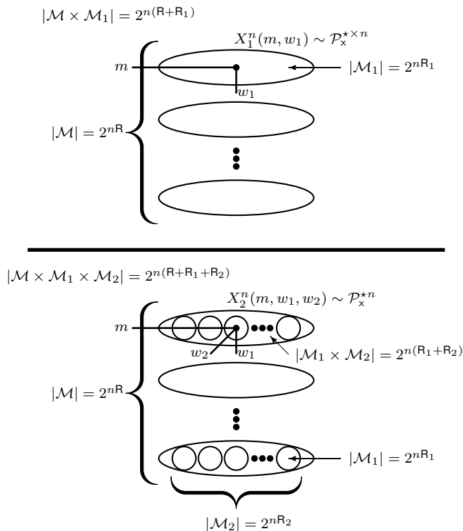
Fig. 14. Binning scheme of the random HARQ-code C \in \mathcal{C}(n, R, L) stated in section A-A for L = 2 transmissions. The parameters n \in \mathbb{N} , R \in \mathbb{R}^+ , R_1 \in \mathbb{R}^+ , R_2 \in \mathbb{R}^+ determine the cardinalities of the set of messages |\mathcal{M}| = 2^{nR} , the cardinality of the bins |\mathcal{M}_1| = 2^{nR_1} and the number of sub-bins |\mathcal{M}_2| = 2^{nR_2} . The random codewords X_1^n(m, w_1) and X_2^n(m, w_1, w_2) are generated with i.i.d. probability distribution \mathcal{P}_x^{*x n} .
