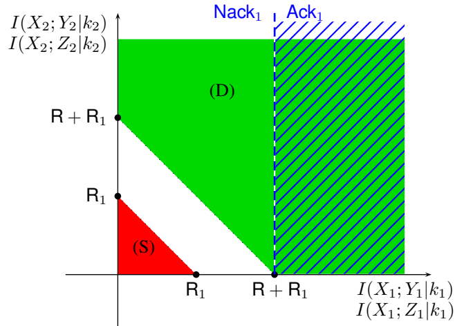
Fig. 4. Regions of correct decoding (D) and secret transmission (S) of [39], corresponding to equations (20) and (21).
