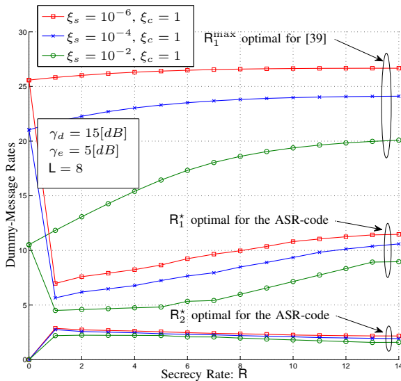
Fig. 11. Optimal rates (R_1^*, R_2^*) for the ASR-code and R_1^{\max} for the protocol of [39], depending on the secrecy rate R under different pairs of constraints (\xi_c, \xi_s) \in \{(1, 10^{-2}), (1, 10^{-4}), (1, 10^{-6})\} .
