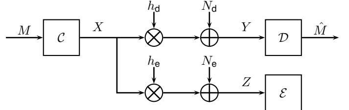
Fig. 7. Gaussian wiretap channel with Rayleigh block fading (h_d, h_e) .
