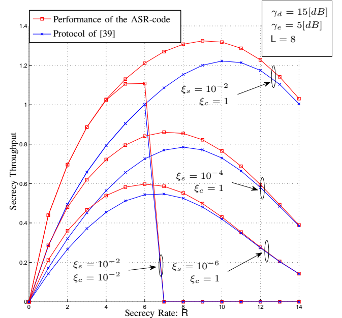
Fig. 10. Secrecy throughput depending on the secrecy rate R , under different pairs of constraints (\xi_c, \xi_s) \in \{(1, 10^{-2}), (1, 10^{-4}), (1, 10^{-6})\} . For each setting, the ASR-code outperforms the protocol of [39].
