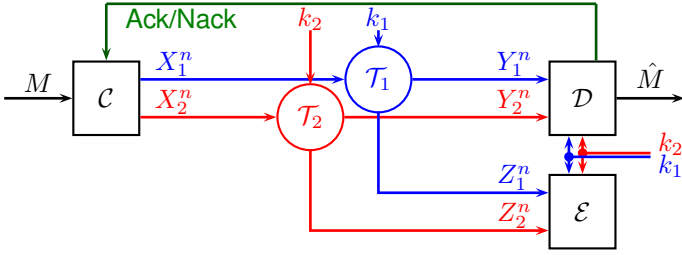
Fig. 1. State dependent wiretap channels \mathcal{T}_i(y_i, z_i|x_i, k_i) , with i \in \{1, 2\} . The second transmission starts if the encoder \mathcal{C} receives a Nack feedback from the legitimate decoder. The state parameters k_1 \in \mathcal{K}_1 and k_2 \in \mathcal{K}_2 are chosen arbitrarily, stay constant during the transmission and are available only at the legitimate decoder \mathcal{D} and at the eavesdropper \mathcal{E} .
