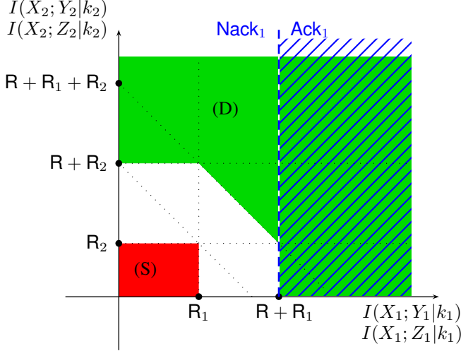
Fig. 5. Regions of correct decoding (D) and secret transmission (S) of [43], corresponding to equations (22) and (23).
