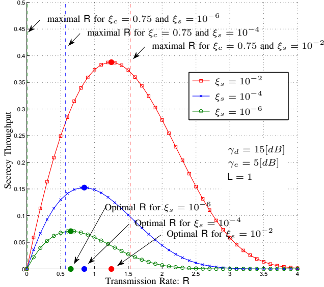
Fig. 8. Secrecy throughput depending on the secrecy rate R \geq 0 , for different secrecy constraints \xi_s \in \{10^{-2}, 10^{-4}, 10^{-6}\} and a single L = 1 transmission. Vertical dashed lines represents the maximal secrecy rate R corresponding to the constraint \xi_c = 0.75 .
