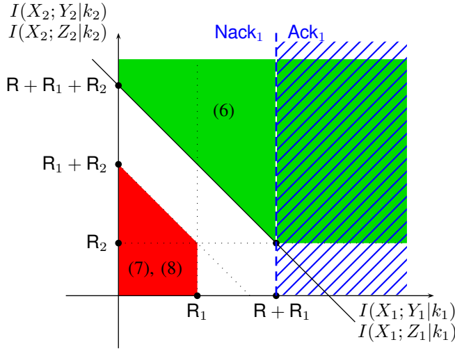
Fig. 2. Decoding and secrecy regions corresponding to the rates (R, R_1, R_2) , for L = 2 transmissions. The second transmission starts only if there is a \text{Nack}_1 , hence we disregard the dashed region of \text{Ack}_1 . The green upper region corresponds to the decoding constraint of equation (6) for the mutual informations I(X_1; Y_1 | k_1) and I(X_2; Y_2 | k_2) . The red lower region corresponds to the secrecy constraints of equations (7), (8) for the mutual informations I(X_1; Z_1 | k_1) and I(X_2; Z_2 | k_2) .
