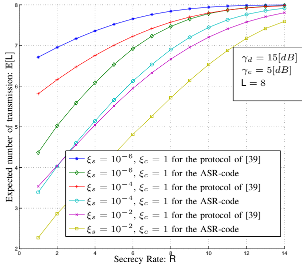
Fig. 13. Expected number of transmissions \mathbb{E}[L] for the ASR-code and for the protocol of [39], depending on the secrecy rate R with different pairs of constraints (\xi_c, \xi_s) \in \{(1, 10^{-2}), (1, 10^{-4}), (1, 10^{-6})\} .
