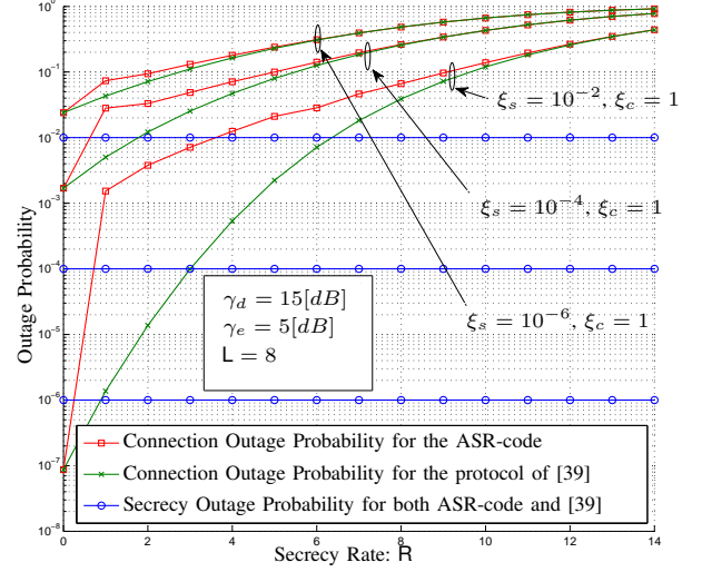
Fig. 12. Connection and secrecy outage probability for the ASR-code and for the protocol of [39], depending on the secrecy rate R under different pairs of constraints (\xi_c, \xi_s) \in \{(1, 10^{-2}), (1, 10^{-4}), (1, 10^{-6})\} .
