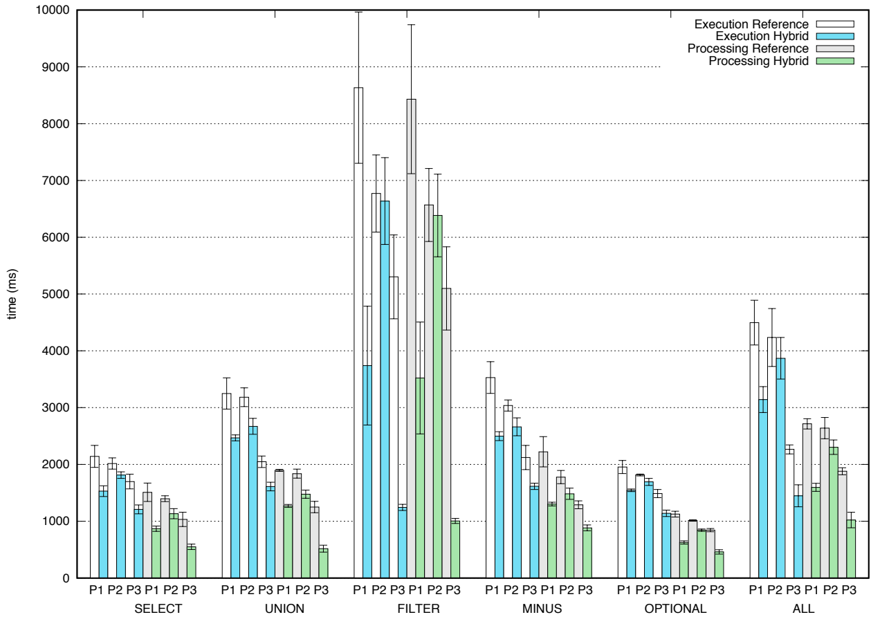
Figure 2: Top: query processing time. Bottom: sub-queries generated
