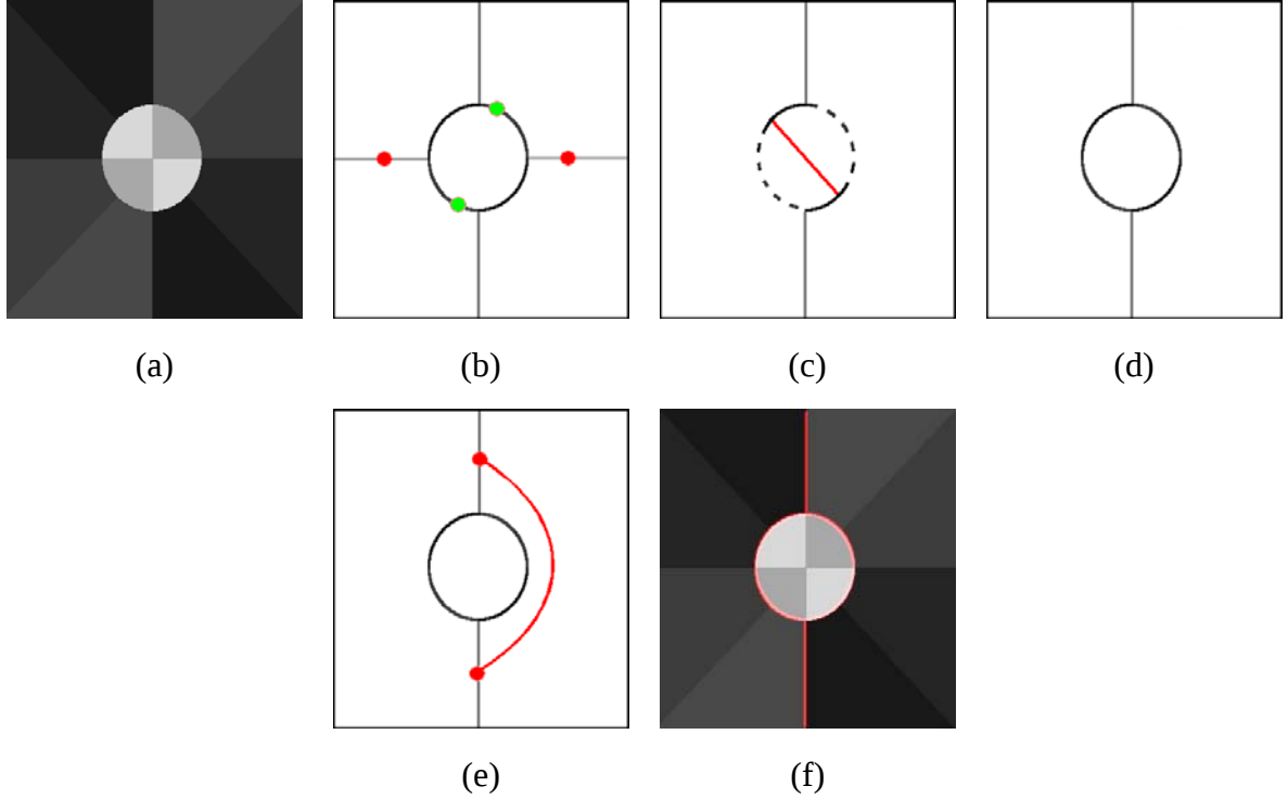
Fig. 62: (a) Initial image, (b) segmentation level s_i with, in red, the minima of h_1 and, in green, two FOZ on the boundary of the central catchment basin. (c) Result of the watershed of h_2 , in red a watershed line marking the central CB as a WSZ (d). (e) and (f), final result, the ground is segmented.
