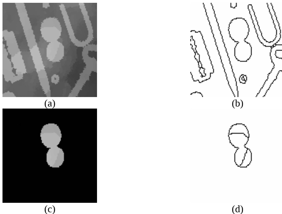
Fig. 69: (a) Detail of TOOLS image, (b) result of P algorithm segmentation on the entire image, (c) focus on the coins (the outside is masked), inner contours become relevant and they appear in a lower level of hierarchy (d).
