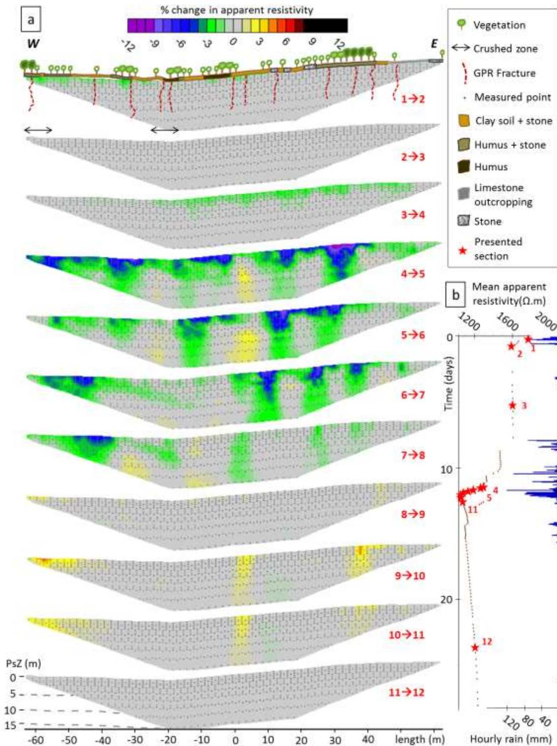
350 Fig. 6: (a) Hourly change in apparent resistivity between two consecutive time steps. Positions of 351 fractures previously detected by ground penetrating radar (GPR) and basic representation of 352 vegetation and soil cover; (b) Evolution of mean apparent resistivity during monitoring versus rain. 353 Each brown point represents one electrical resistivity tomography section (Carrière et al. 2015). PsZ is 354 pseudo depth. 355
