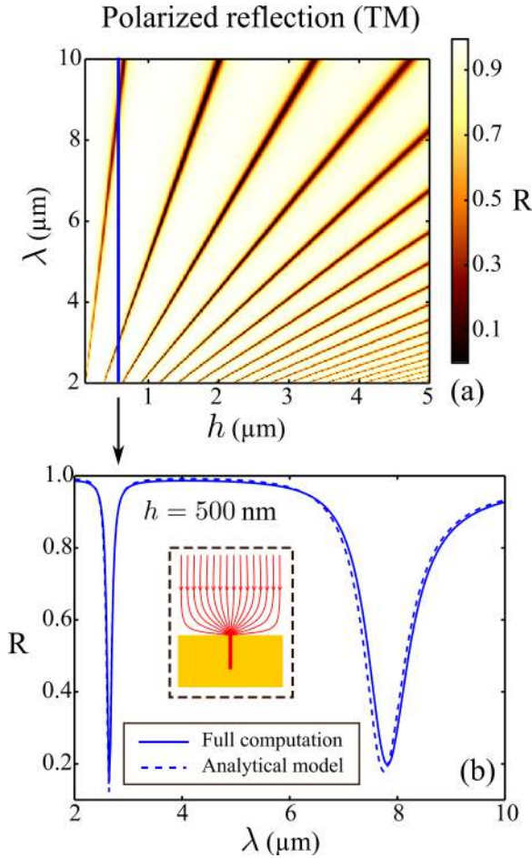
FIG. 4. (a) Reflectivity map as a function of the wavelength \lambda and the thickness h for the reflection. (b) Reflectivity as a function of the wavelength \lambda at a selected h = 500 nm. The dashed line represents the result obtained with the effective-medium model and the solid line shows the full computation with the original resonator. The parameters are w = 200 nm and d = 1 \mu\text{m} . The dielectric is gallium arsenide and the metal is gold.
