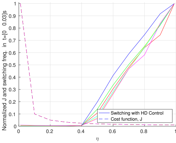
Fig. 4. Evolution of the normalized switching frequency w.r.t. \eta for different initial conditions in the inverter.
