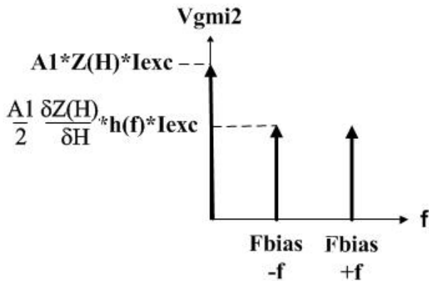
Figure 7. Frequency domain of GMI signal ( V_{gmi2} ) after multiplication by clock at f_{exc} .
