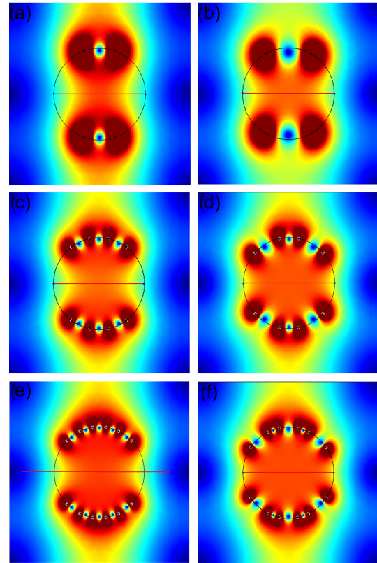
Figure 7. Magnetic field homogeneity of the Everett–Bolinger coil: (a), (c) and (e), respectively, for two, four and six turns. The SHS coil: (b), (d) and (f), respectively, for two, four and six turns.
