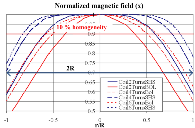
Figure 8. Magnetic field homogeneity profile on the x axis, comparison between Everett–Bolinger coil and SHS coil for two, four and six turns.
