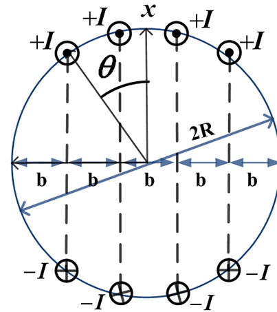
Figure 4. Bolinger's coil: the turns, distributed along the circumference (placed around the cylinder at angles \theta (NB the complementary angle \Phi was used in Bolinger's paper)), are equally spaced projected along the diameter ( b = 2R/(2N + 1) ).
