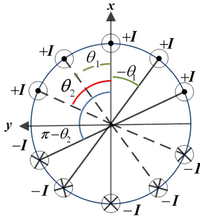
Figure 5. Electrical conductors of unknown angular positions ( \theta ), flown by the same current I , distributed along the circumference.
