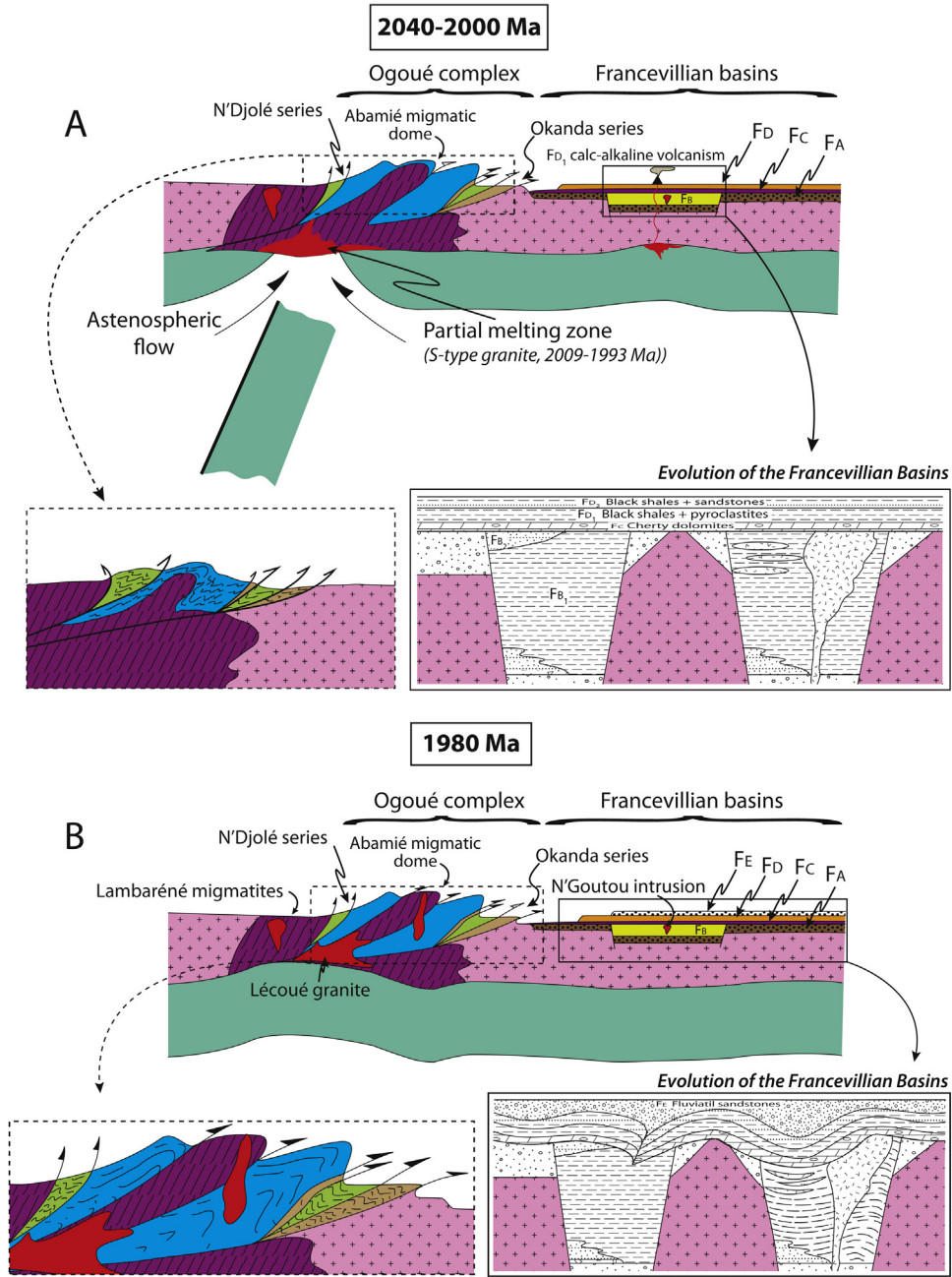
Fig. 5. Conceptual model for the evolution of the Eburnean orogeny in the mobile zone of Ogooué and consequences in sedimentation and magmatic activity in the Francevillien basins (end). A. The continental collision, stop of the subduction (2040 to 2000 Ma). The fast rise of the Ogooué Complex might be the result of a slab break-off. The metamorphic and unmetamorphosed units are thrust toward the northeast. A hot asthenospheric flow linked to the slab break-off leads to partial fusion within the middle to lower crust, generating the Lécoué granite, which seals the tectonic units of the Ogooué complex. The subsidence of the Francevillien basins ceases to be active and the basins are filled. The FC formation corresponds to a quasi-emersion of the basin. The alkaline magmatic activity in the Okondja basin ceases. After the emersion of the FC, the important transgression FD covers the whole region, after a general collapse of the foreland of the Ogooué complex. The calc-alkaline magmatism observed at the base of the FD formation (FD1) results from partial fusion along deep lithospheric faults. B. At the end of the Eburnean orogeny, the post-collisional adjustments (rotation of blocks) occurring 1950 Ma ago cause important deformations in the basins (mainly in the Okondja basin) and are responsible for the overall emersion. The final erosion of the reliefs produces the FE sandstones.
