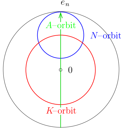
FIGURE 5. Ball model of \mathbb{H}^n
