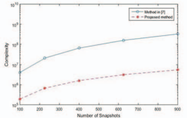
Fig.2. Complexity Comparison with Different Number of Antenna Elements ( L=200 )
