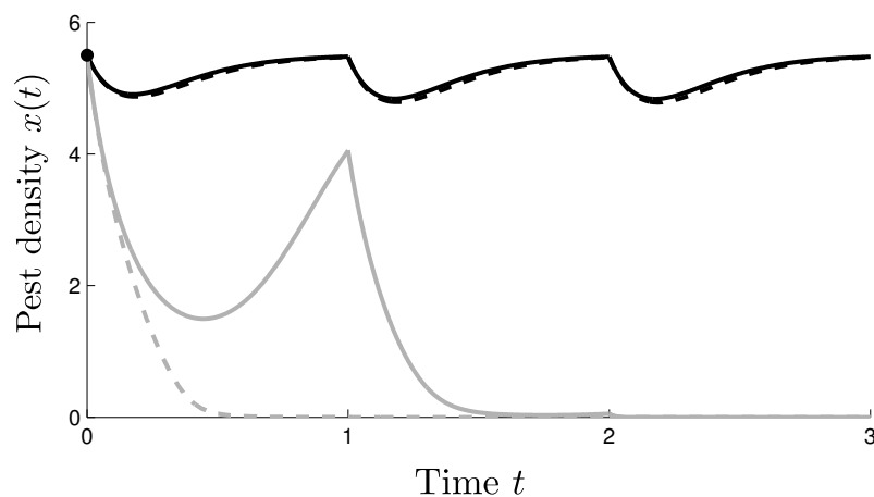
Fig. 2 Comparison of the four models pest-dynamics with \mu = 4 , T = 1 and parameters used in Figure 1. Black curves represents pest densities when foraging efficiency Allee effects occur among predator (solid curve: RF-model, dashed curve: F-model). Gray curves represents pest densities of the R-model (solid curve) and RMA-model (dashed curve).
