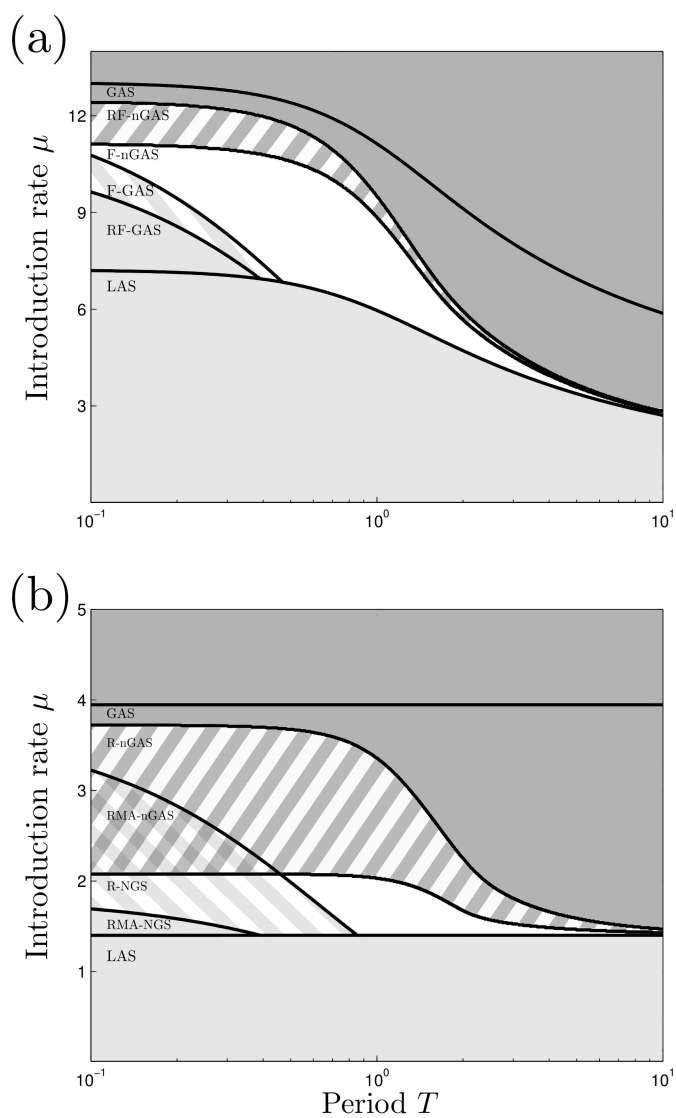
Fig. 1 Stability conditions of pest-free solution as functions of T (in logarithmic scale) and \mu . The RF- and F- models are compared in (a) while R- and RMA- models are studied in (b). The numerical stability (see text) and NGS regions are represented by dark gray and light gray colors, respectively. In the top dark gray area, both models are analytically GAS while in the bottom one, they are numerically stable. In the dark gray hatched area, only the F-model and RMA-model are numerically stable in (a) and (b), respectively. In the bottom light gray area, both models are unstable while in the top light gray area, they are NGS. In the light gray hatched area, the F- (RMA-) and RF- (R-) models are LAS and NGS in (a) (in (b)), respectively.
