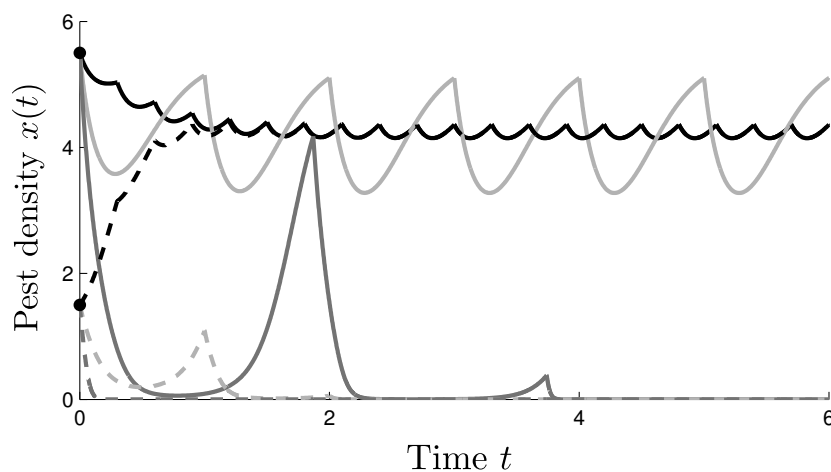
Fig. 3 Influence of period T and initial condition for pest control success on pest dynamics in the R-model. Parameters the same than in Figure 1 with \mu = 2.5 . The initial condition used for dashed and solid solutions are (1.5, \mu T) and (K, \mu T) , respectively. T = 0.3 is illustrated in black, T = 0.8 in light gray and T = 1.9 in dark gray.
