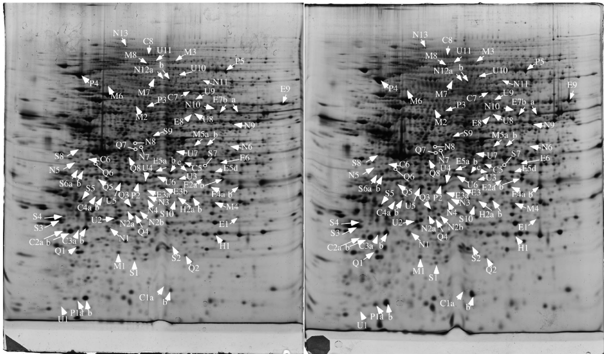
Figure 3: Proteomic analysis of total cell extracts by 2D electrophoresis: effect of culture medium
