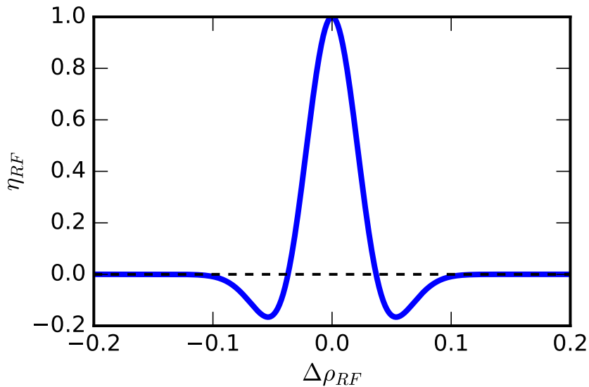
Figure 11: Efficiency \eta_{RF} , as approximated by equation 16, with \alpha = 0.037 and \beta = 0.039 .
