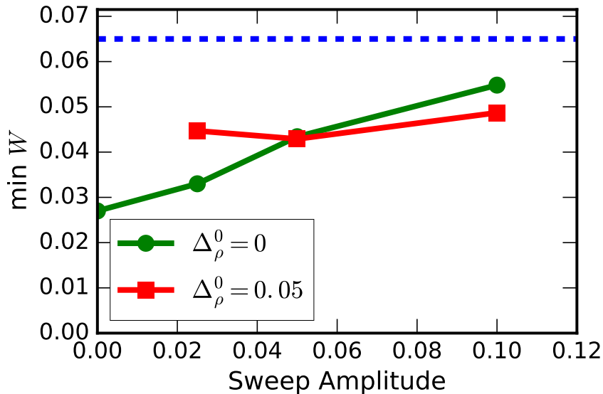
Figure 10: Saturation width reached as a function of sweeping amplitudes, for different misalignment of the sweeping. The dash line indicates the saturated width of the island.
