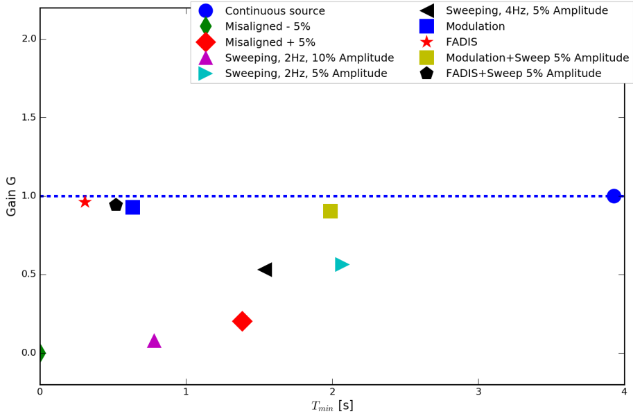
Figure 15: Gain function as a function of the time T_{min} necessary to reach the minimum island width, obtained with thin source term ( \delta_{RF} \approx 0.7W_{sat} ). Notice how the sweeping allows increasing the gain with respect to a misaligned source, while being less efficient than a perfectly aligned source
