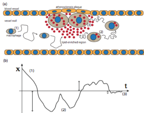
Figure 1: a) Sketch of the different stages of atherosclerosis plaque formation: (1) rapid diffusion of a free macrophage cell; (2) upon entering a localized lipid-enriched region, the macrophage accumulates lipids, and thereby grows and becomes less mobile; and (3) after many crossings of the lipid-enriched region, the macrophage eventually gets trapped, resulting in the formation of an atherosclerotic plaque. (b) Sketch of a one-dimensional particle trajectory of the model of locally decelerated random walk.
