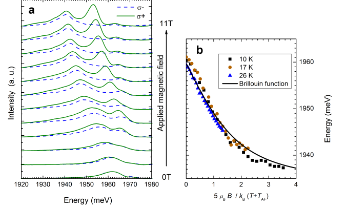
Figure 5. Magneto-optical spectroscopy.
