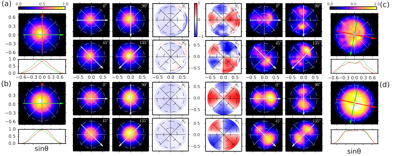
Figure 3. Coordinate system is the same as in Fig 1(c). In each panel we present the normalized unpolarised far field radiation diagram with two cross sections along the direction of the red and green arrows, the linearly polarised radiation diagrams at \{0^\circ, 90^\circ\} and \{45^\circ, 135^\circ\} sharing the same normalization factor (direction of polariser is indicated by gray arrow), and the S_1 and S_2 stokes parameter maps. (a), experimental results for the ZnTe emission line. (b), corresponding simulation results ( \rho/\Delta_{LH} = 0.14 , \sigma/\Delta_{LH} = 0.24 , \psi = 112^\circ , \chi = 186^\circ , or conversely \rho_0/\Delta_{LH0} = 0.14 , \hat{\alpha} = 100^\circ , \hat{\beta} = 5^\circ and \hat{\gamma} = 12^\circ ). (c), experimental results for the QD emission line. (d), corresponding simulations ( \rho/\Delta_{LH} = -0.23 , \sigma/\Delta_{LH} = -0.06 , \psi = 170^\circ , \chi = 137^\circ , or conversely \rho_0/\Delta_{LH0} = -0.23 , \hat{\alpha} = 20^\circ , \hat{\beta} = 16^\circ and \hat{\gamma} = 150^\circ ).
