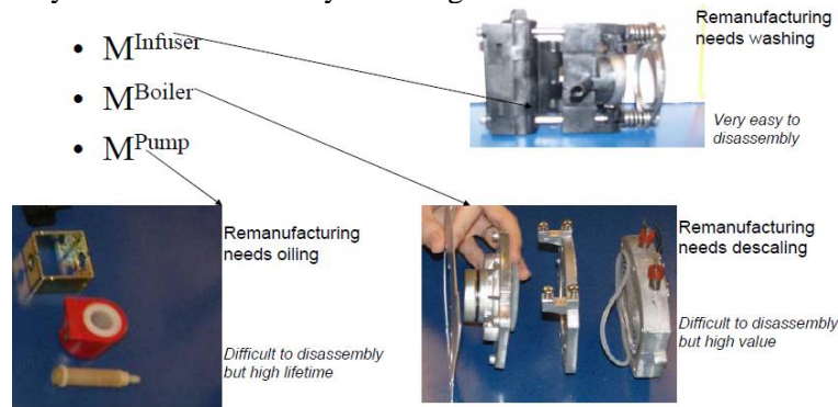
Figure 5. Modules characteristics
