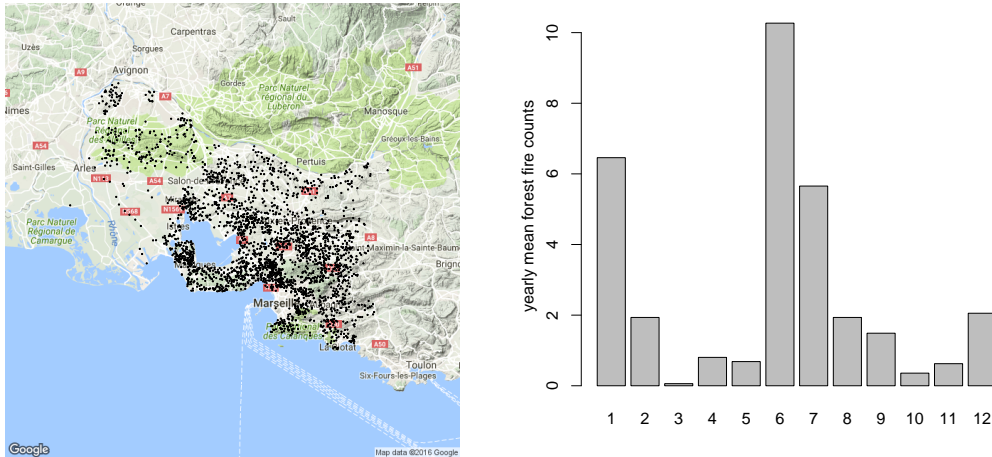
FIGURE 1. Left: Map of forest fire locations recorded in the Bouches-du-Rhône department in Southern France. Right: Mean yearly number of forest fires with burnt surface superior to 1ha with respect to months.
