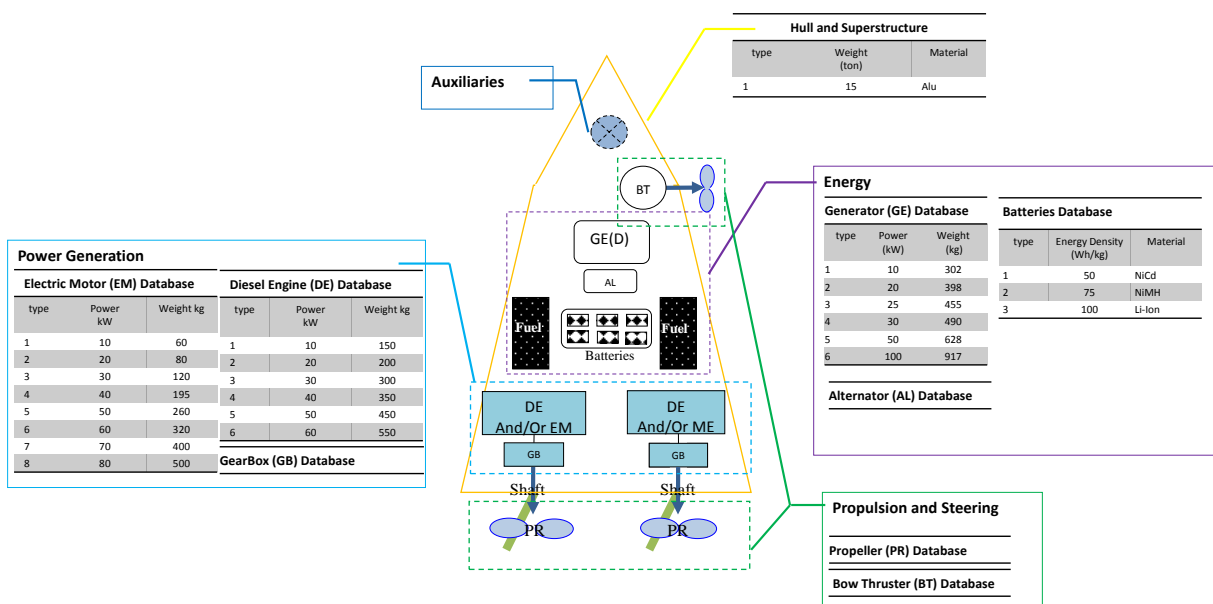
34 35 Figure 4: Model of hybrid passenger ferry.
