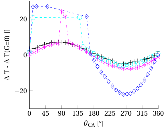
Figure 9: Evolution of the temperature gradient for a given heat supply of 70 \text{ W} and several values of gain: G = 2.0 (+) , G = 3.0 (*) , G = 3.2 (o) or G = 10 (diamond) .
