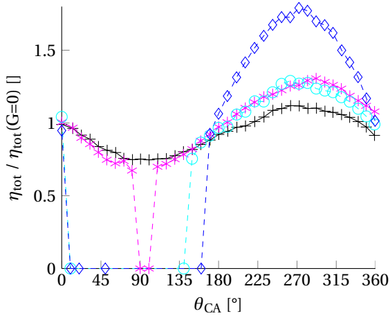
Figure 8: Evolution of the normalized efficiency for a given heat supply of 70 \text{ W} and several values of gain: G = 2.0 (+) , G = 3.0 (*) , G = 3.2 (o) or G = 10 (diamond) .
