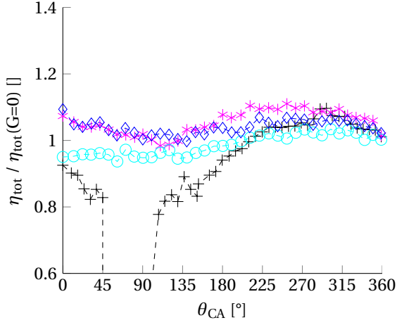
Figure 6: Evolution of the normalized efficiency with the variation of the phase-shift for a heat supply \dot{Q}_h = 70 \text{ W (+)} , 80 \text{ W (*)} , 90 \text{ W (o)} or 100 \text{ W (diamond)} and a constant gain G = 1 .
