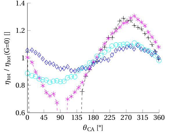
Figure 7: Evolution of the normalized efficiency with the variation of the phase-shift for a heat supply \dot{Q}_h = 69.9 \text{ W (+)} , 70.5 \text{ W (*)} , 80 \text{ W (o)} or 110 \text{ W (diamond)} and a constant gain G = 3.2 .
