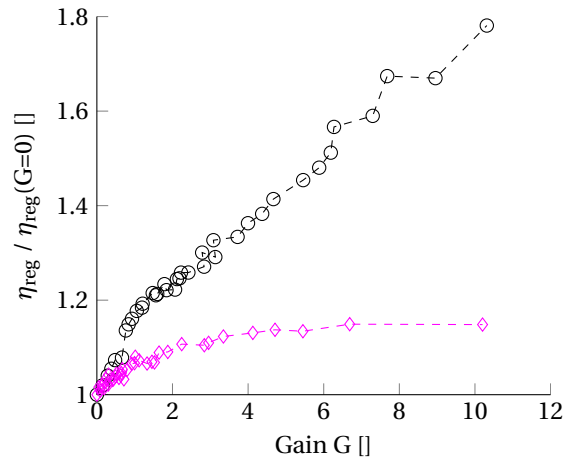
Figure 11: Evolution of the efficiency with the variation of the power supplied to the auxiliary source, for a given heat supply of 70 W (o) or 140 W ( \diamond ) and a constant 90^\circ -phase-shift.
