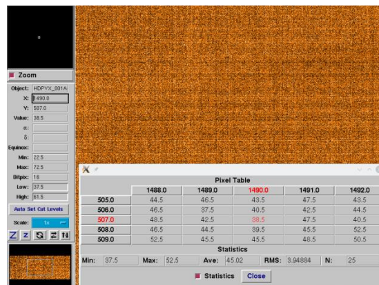
Fig. 9. left) HDPYX dark image in High gain configuration showing 4 ADU RMS corresponding to attended 2.5e read out noise.
