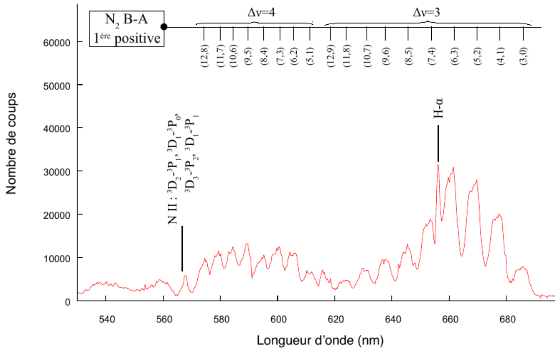
Fig. 1. Spectrum of the auroral simulator planeterrella (ref papier Jean) between 520 and 700 nm. The resolution is around 1 nm. The spectrum of the aurora is somehow different since forbidden transitions also appear in aurora and airglow mainly O 1 S at 557 nm and O 1 D triplet at 630, 639 and 639 nm
