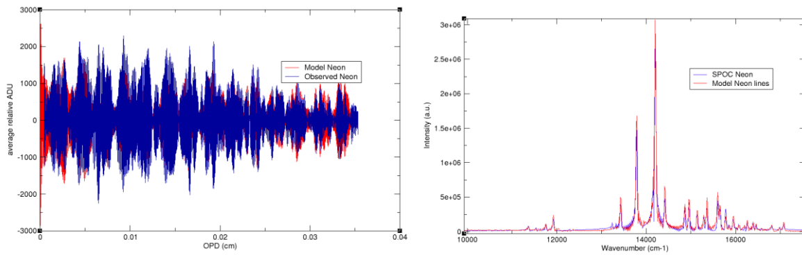
Fig. 8. left) Reconstructed interferogram. Only the positive part of interferogram is measured. right) reconstruction of neon spectra surimposed to theoretical neon spectra.
