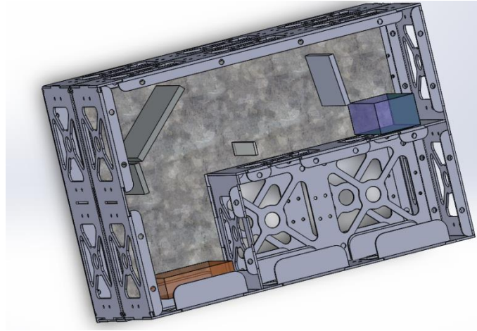
Fig. 3. ATISE Mechanical implementation for optical test assembled with 6U platform.
