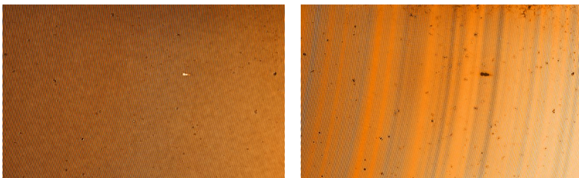
Fig. 7. left) Observed Fringes of neon's 703nm spectral line on SPOC; right) Observed fringes of whole neon's spectra
