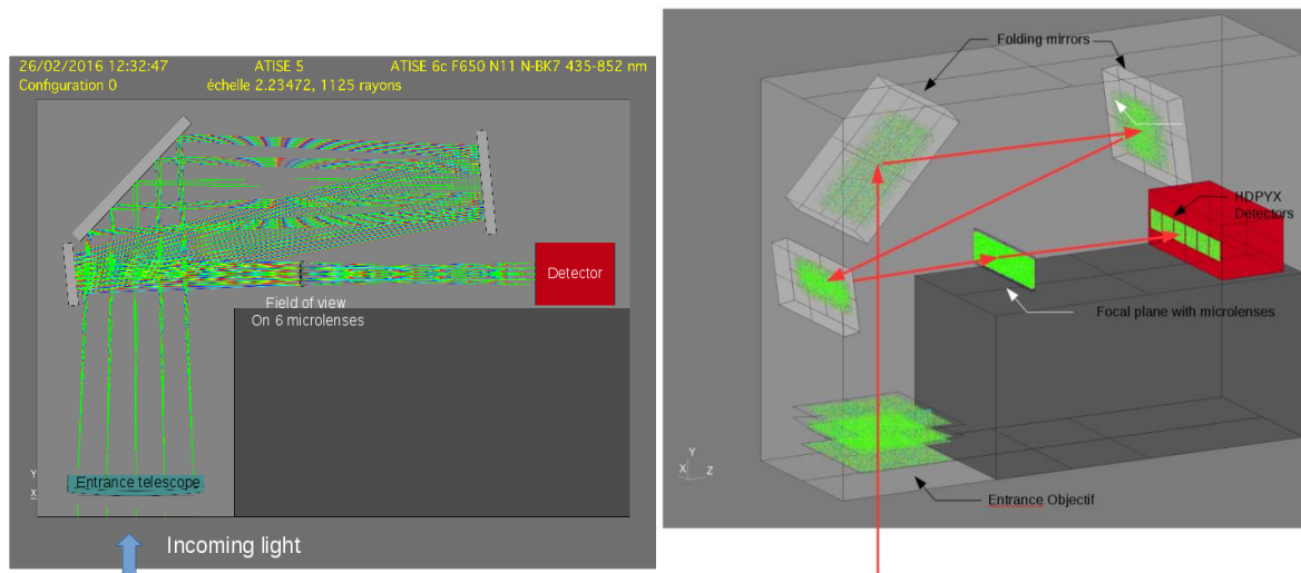
Fig. 4. a) ATISE optical schematic. b) Perspective view showing light distribution on each optical surface. The optics forms an image of entrance pupil on detector which create an uniform illumination corresponding to one of six line of sight.
