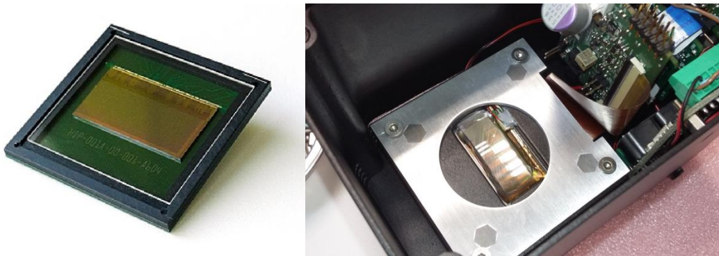
Fig. 6. left) Pyxalis HDPYX Sensor in BGA, Ceramic Ring configuration; right) tested SPOC configuration , a 60nm TiO2 layer has been deposited on plane of plano-convex lens. An optical fiber is set at focal plane of the lens to obtain flat illumination.
