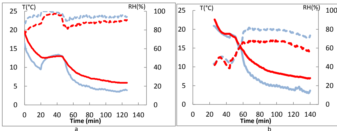
Figure 2: Evolution of the air temperature and relative humidity for the air return of the evaporator and for air blown by it a- without dehumidifier b-with dehumidifier
