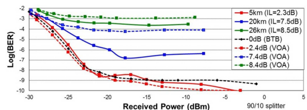
Fig. 2: BER transmission performances versus received power at 2.5Gbps, for standart self-seeded with different cavity length and their equivalent attenuation using a VOA (dashed curves)
