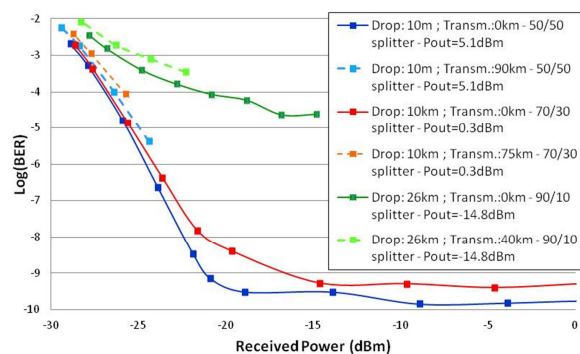
Fig. 4: 2.5Gbps BER transmission performances versus received power, for 10m cavity (blue), 10km cavity (red/orange) and 26km cavity (green) for various feeder fiber length
