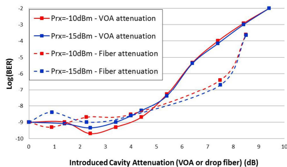
Fig. 3: Comparison of the BER transmission performances versus introduced cavity attenuation for a given received power at 2.5Gbps
