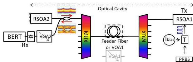
Fig 5: Experimental setup of the RSOAs “face-to-face” self-seeded
