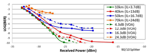
Fig. 6: BER transmission performances versus received power at 2.5Gbps, for RSOAs “face-to-face” self-seeded with different cavity length and their equivalent attenuation using VOA (dashed)
