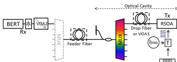
Fig. 1: Experimental setup of the “regular” self-seeded
