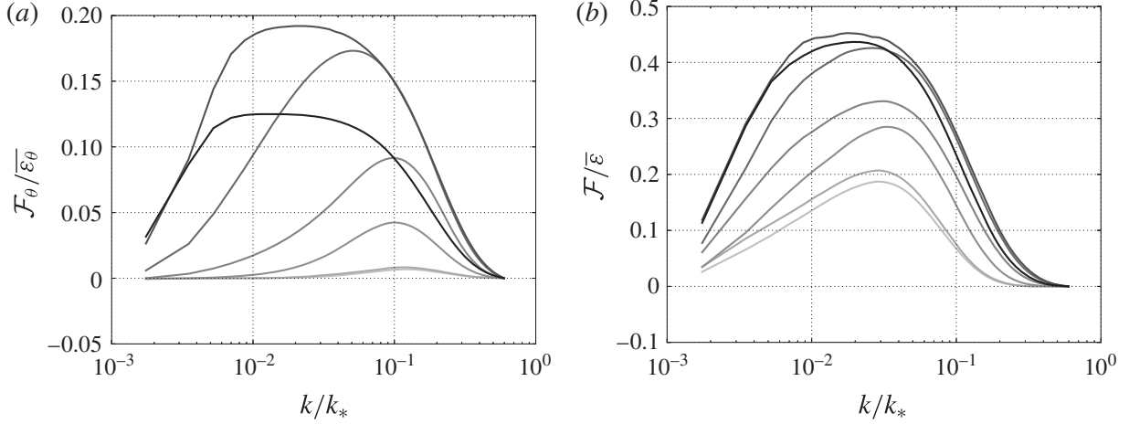
FIGURE 16. Temperature flux \mathcal{F}_\theta(k) (a) and turbulent kinetic energy flux \mathcal{F}(k) (b) for the different Stokes numbers and for ( St=0.003, 0.019, 0.074, 0.352, 1.064, 7.343 and 29.36 , from light grey to black respectively) at \gamma=570 , C=0.19 . Both quantities are normalized by the mean rate of dissipation of the temperature fluctuations \overline{\varepsilon}_\theta and the mean rate of dissipation of turbulence \overline{\varepsilon} , respectively.
