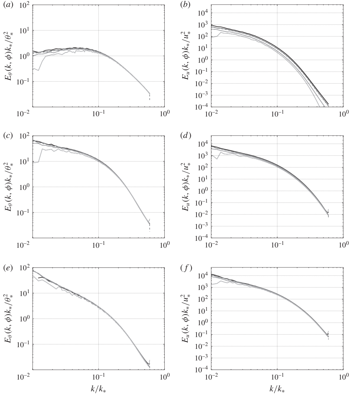
FIGURE 17. The anisotropic spectra of the temperature fluctuations ( a,c,e ) and of the turbulent kinetic energy ( b,d,f ) for St=0.003 ( a,b ), 0.352 ( c,d ) and 7.343 ( e,f ) at \gamma = 570 , C = 0.19 , for four values of \phi : \phi = \pi/2 , \phi = \pi/3 , \phi = \pi/5 and \phi = 0 , from light grey to black respectively. Comparison with the global spectra in grey dashed lines.
