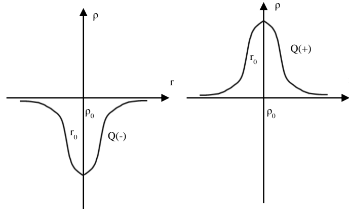
Fig. (1) A Charge and its Field
