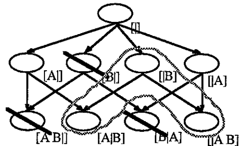
Figure 6. The graph of Figure 5 where the environments in which B holds are inconsistent. So, three of the environments are inconsistent ( [B] , [B|A] and [B A] ) and only three of them can be included in labels: [A|B] , [A B] and [A B] (those for which every completion is consistent; they are represented surrounded with a dotted line).
