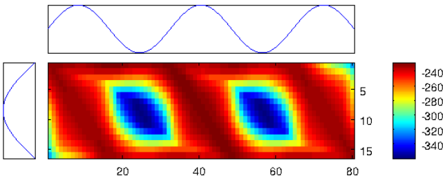
Fig. 2. Forward Backward matrix (logarithmic values) for the alignment of a positive halfwave with a sinus wave. The dark red color represents high probability states, while dark blue color represents low probability states.
