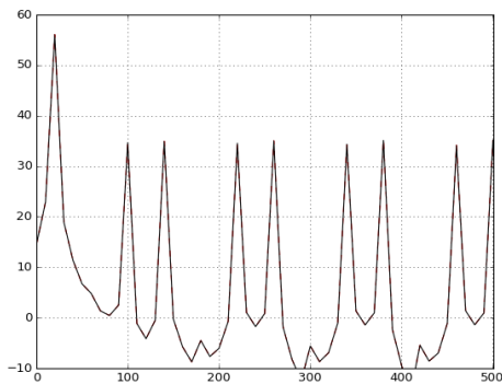
Fig. 5. Log power spectra of a \tilde{X}_k component.
