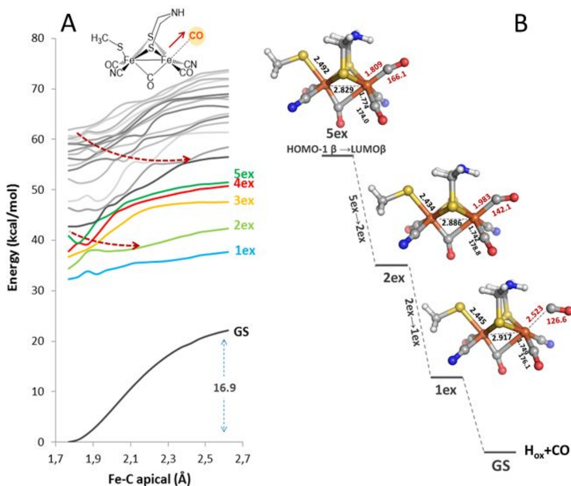
Figure 4. Panel A: potential energy surfaces of the ground state and the first 20 excited doublet states of \text{Fe}_2\text{S}_2 \text{H}_{\text{ox}}\text{-CO} model along the apical Fe-C stretching coordinate. Energy differences in kcal/mol, computed with respect to the minimum ground state energy. The value of the free energy dissociation barrier is also reported, and compares well with the experimental value determined in experiments shown in Supplementary Fig. 20. Red arrows guide the eye to follow the dissociation pathway through the surface crossings. Panel B: geometry optimized structures for the \text{Fe}_2\text{S}_2 fifth (5ex) excited state, along the CO dissociation pathway. Distances in Å, angles in degree.
