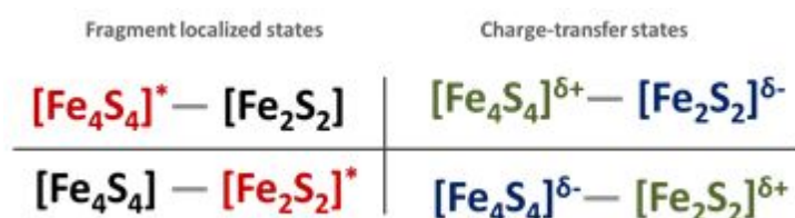
Scheme 1. H-cluster electronic excitation resulting from frontier MO composition. From left: fragment localized (in red) states (on \text{Fe}_4\text{S}_4 or \text{Fe}_2\text{S}_2 ), and \text{Fe}_4\text{S}_4 \rightarrow \text{Fe}_2\text{S}_2 / \text{Fe}_4\text{S}_4 \rightarrow \text{Fe}_2\text{S}_2 charge transfer states.
