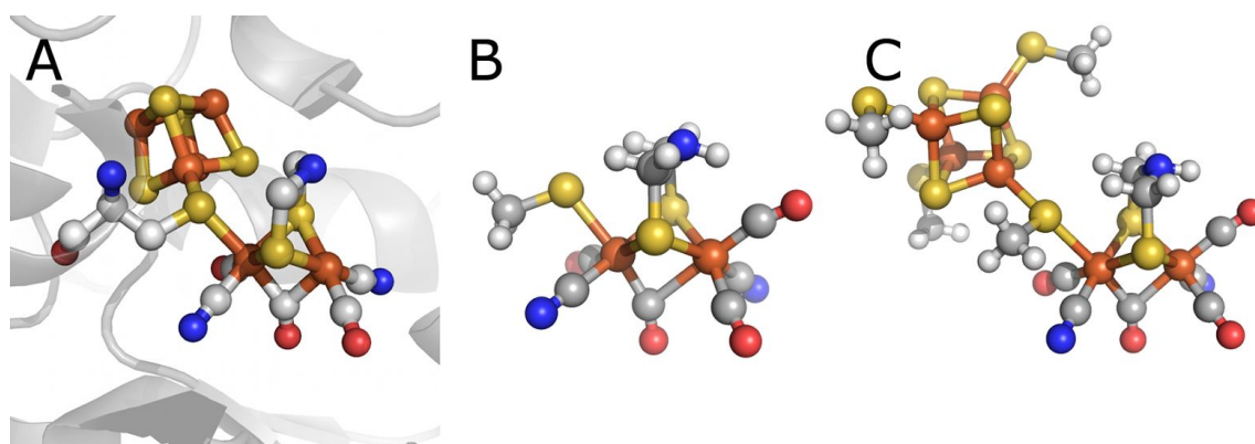
Figure 1. The H-cluster of hydrogenase. Panel A: the structures of the active site of C. acetobutylicum FeFe hydrogenase, adapted from pdb 3C8Y. 23 Panels B and C: the two models of H_{ox} -CO used in our TDDFT calculations.
