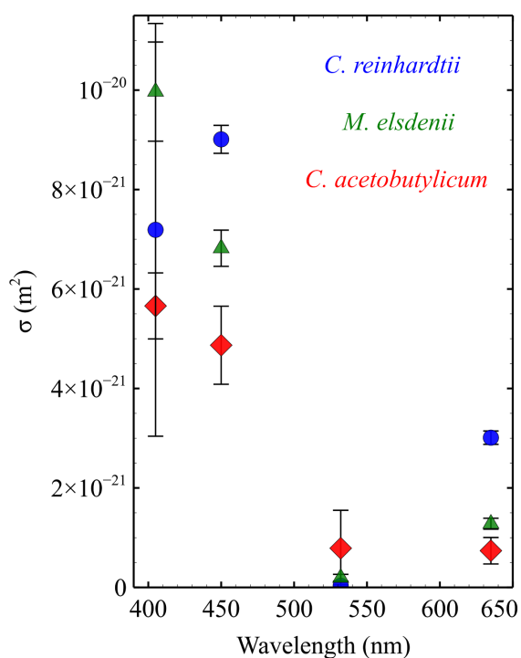
Figure 3. Dependence on wavelength of the effective cross section for the photodissociation of CO (calculated from the slope of the line in fig 2D multiplied by h\nu ) on the rate of CO release from the active site of the FeFe hydrogenases from C. reinhardtii (blue), C. acetobutylicum (red) and M. eldensii (green).
