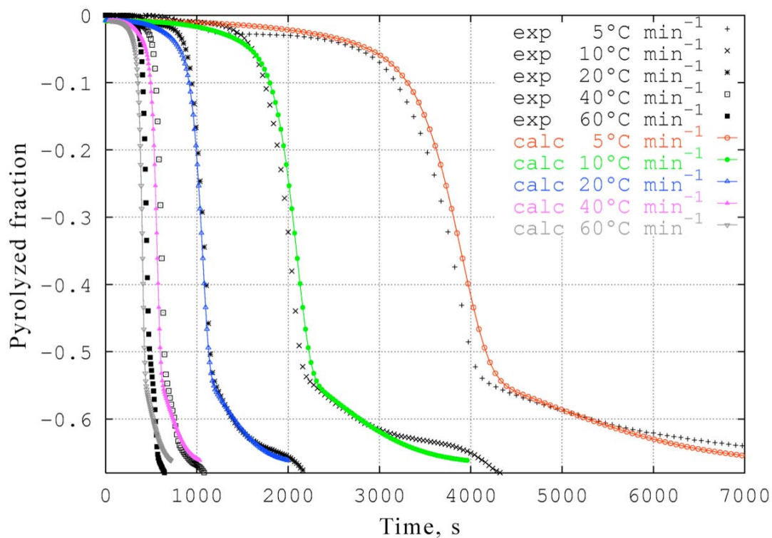
Figure S1. Comparison between experimental mass-loss curves and those calculated from the model of Garcia et al. Obtained from Menard. 2
