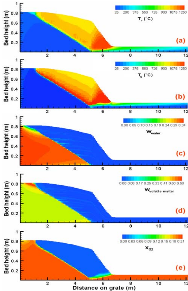
Figure 4. Main results from the model: (a) Temperature of solid, (b) temperature of gas, (c) mass fraction of moisture in the solid, (d) mass fraction of volatile matter in the solid and (e) mole fraction of oxygen in the gas phase.
