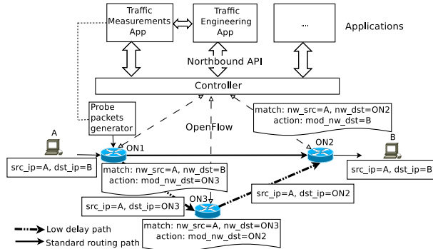
Figure 1: Overlay architecture
