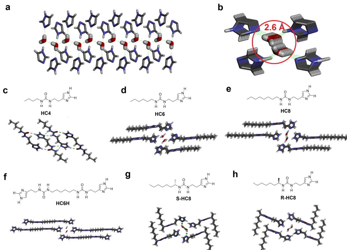
Figure 1. Artificial I-quartet water channels and their chiral isomers pack differently. a. Side and b. top views of I-quartet water/proton channels that self-assemble into tetrameric- tubular architectures confining dipolar oriented water-wires. Top views of water confining I-quartet channels in stick representations (N, blue; C, grey; O, red; H, white), taken from crystal structures of C. Butylureido-ethylimidazole HC4 , D. Hexylureido-ethylimidazole HC6 , E. Octylureido-ethylimidazole HC8 , F. Bis(ethylimidazole ureido)hexyl HC6H , 11 G. S-Octylureido-ethylimidazole S-HC8 and R-octylureido-ethylimidazole R-HC8 . These structures show that packing and self-assembly are dramatically different between chiral and achiral isomers, but all channels have pores with a diameter of 2.6 Å.
