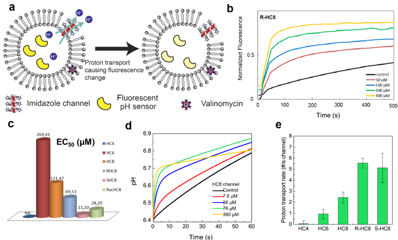
Figure 3. Proton-transport activity of I-quartet channels in liposomes. a. Liposomes encapsulating pH-sensitive dyes (8-hydroxypyrene-1,3,6-trisulfonic acid [HPTS] and fluorescent dextran) showed fluorescence quenching because of proton export via imidazole channel and K^+ import via Valinomycin channel (see Supplementary materials for details). b. Ratiometric fluorescence ( I/I_0 ) curves of the assembled R-HC8 channels with different channel concentrations in the HPTS assay. The signal was normalized at t=500 s. c. Calculated values of EC_{50} (in \mu M) determined in the HPTS assay, representing the concentration at which the given compound (including racemic RacHC8 ) achieved half of its total transport capabilities. d. The pH inside the liposomes (pH=6.4) with the incorporated HC8 channels increased over time upon exposure to a higher pH environment (pH=7.4) in kinetic experiments. The experiments were performed on a stopped-flow instrument using a fluorescent D-3305 dextran dye as a pH sensor. Higher HC8 channel concentrations correlated with faster transport kinetics. e. Proton-transport rates of different I-quartet channels calculated from the fluorescent dextran assay. The data shown are the averages of at least triplicates, and the error bars represent the standard deviation.
