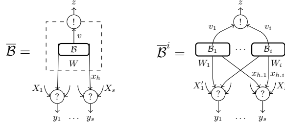
Fig. 9: i -ary box expansion.
