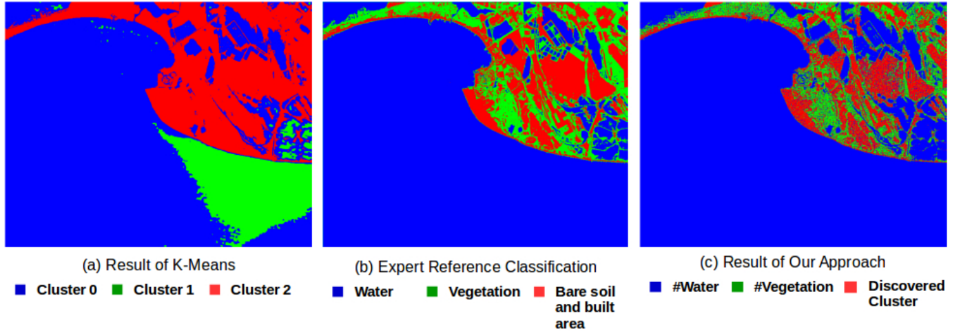
Fig. 8. Results of k-means (a) and our approach (c) compared with an expert reference classification of an excerpt of a Landsat scene of the south of France
