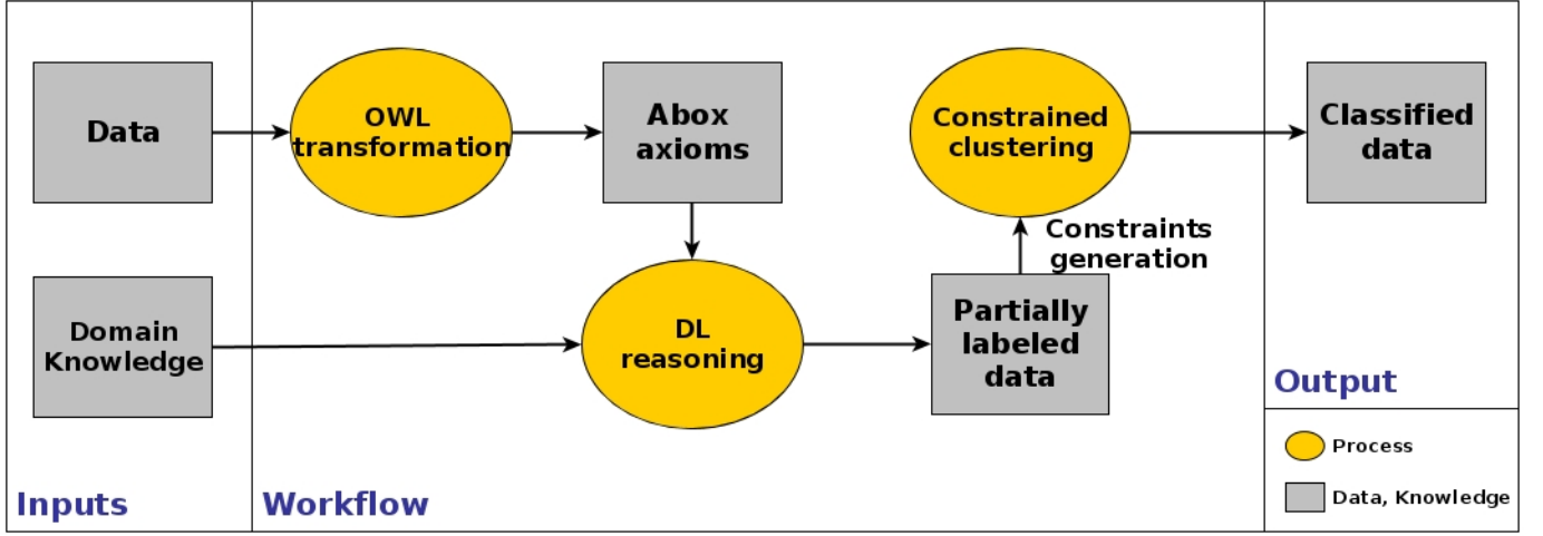
Fig. 1. Overview of Our Approach
