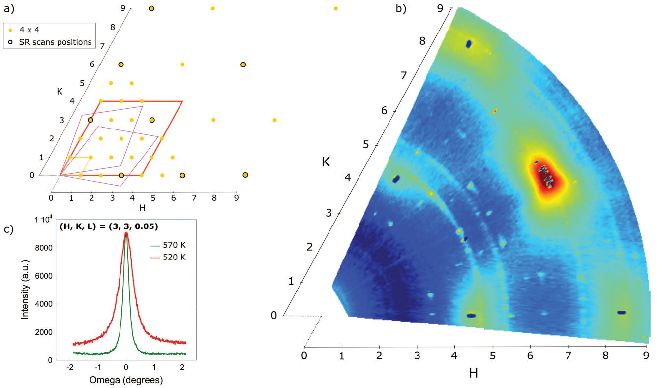
Figure 1. a) Schematics of the measurements performed at 520 K and 570 K. The indexing of the axis refers to the (4 \times 4) reconstruction. The yellow, pink and red parallelogram represent the (4 \times 4) , (1.338 \times 1.338) R \pm 10.02^\circ and Ag(111) unit cells, respectively. Yellow disks indicate the position of in-plane rocking scans, whereas black circles indicate the position of the analyzed rods. b) In-plane map ( L=0.05 ) of the reciprocal space obtained by GIXD measurements at 570 K. c) Rocking scan performed around (H, K, L) = (3, 3, 0.05) at 520 K (red line) and 570 K (blue line). The almost identical intensity at \omega = 0 is fortuitous.
