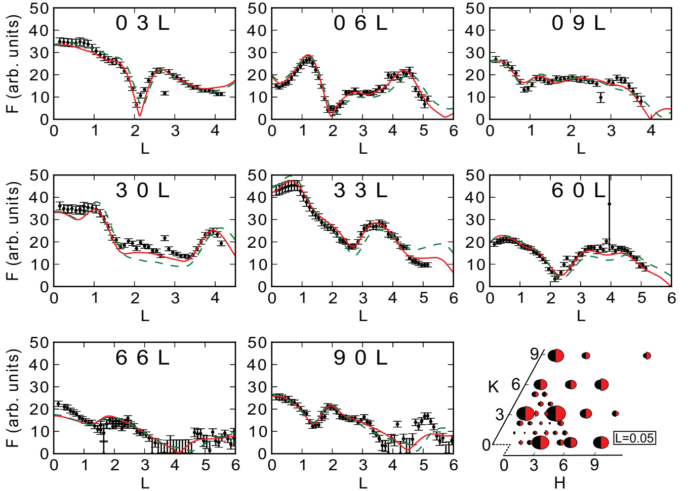
Figure 3. Comparison between experimental, for T = 520\text{K} , (black dots with error bars and black half-disks), GGA-simulated (red continuous line and red half-disks) and LDA-simulated (green dotted line) structure factors, along several superstructure rods and for in-plane diffraction conditions ( L = 0.05 ).
