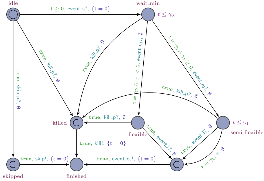
Figure 8: Timed automaton modelling a flexible temporal relation with minimum duration \gamma_0 and maximum duration \gamma_1 . \gamma_1 < 0 means that the maximum duration is infinity while \gamma_1 \geq 0 means that it is bounded.
