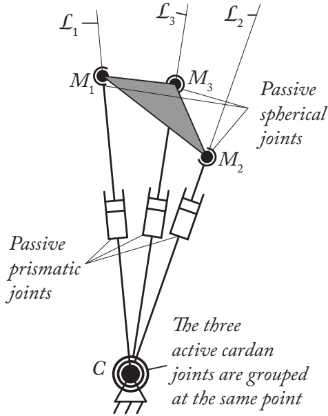
Fig. 4. The hidden robot model: a 3- \underline{UPS} parallel robot with all active cardan joints merged at the point C (for reason of clarity of drawings, the axes of the cardan joints are not represented)
