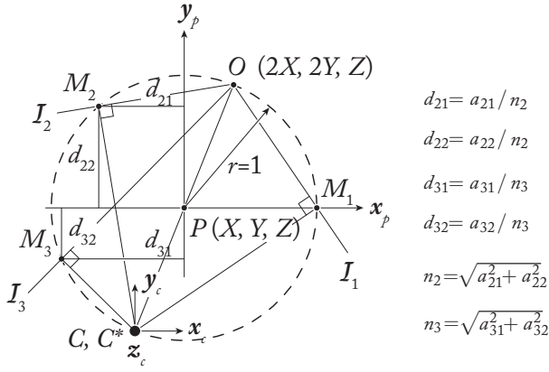
Fig. 10. Parameterization of the location of the three observed points.
