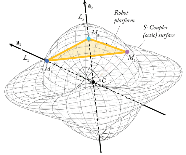
Fig. 5. The octic surface (coupler surface, i.e. the surface which represents all possible location of the extremity of the “coupler” which is the body linking the disconnected leg to the rest of the mechanism) representing the displacements of point M_3 when the lines \mathcal{L}_1 and \mathcal{L}_2 are fixed in space: in this figure, \Delta M_1M_2M_3 is an equilateral triangle of edge length equal to 2\sqrt{3} m. Moreover, we have \mathbf{a}_1^T \mathbf{a}_2 = 5/8 , \mathbf{a}_i being the unit vector representing the direction of the line \mathcal{L}_i .
