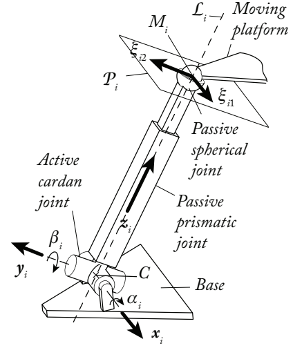
Fig. 3. A \underline{UPS} kinematic chain
