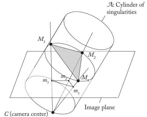
Fig. 1. Cylinder of singularities found in [2].
