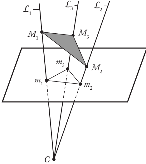
Fig. 2. Observation of three 3-D points
