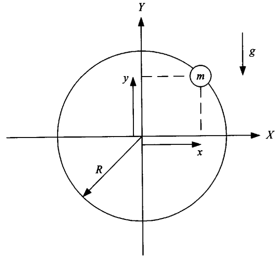
Fig. 1 A bead of mass, m , moving on a circular ring of radius, R
