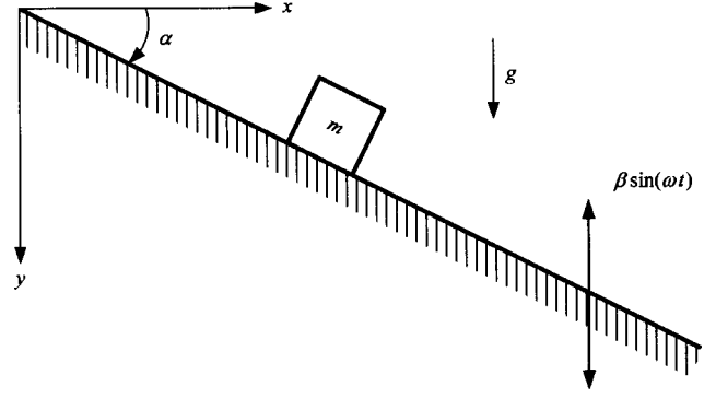
Fig. 2 A block sliding under gravity on an inclined plane ( 0 < \alpha < \pi/2 ) that is vibrating vertically with amplitude \beta and frequency \omega . The coefficient of Coulomb friction between the plane and the block is \mu .
