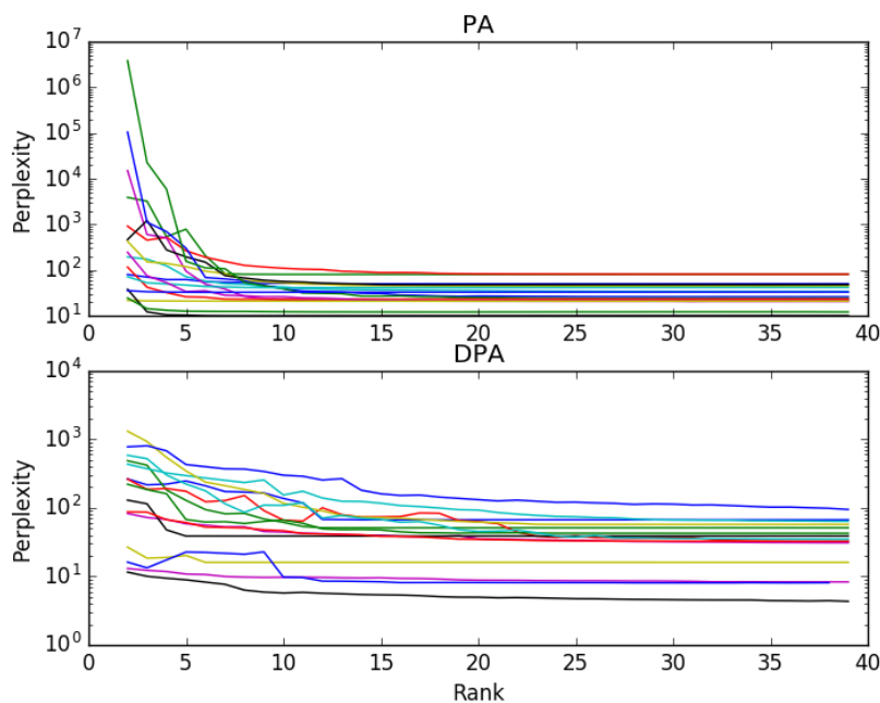
Figure 2: Perplexity evolution with the rank on problems whose targets are Probabilistic Automata (top) and Deterministic Probabilistic Automata (bottom). Each line corresponds to one given set of parameters (values of version , lrows , lcolumns ).
