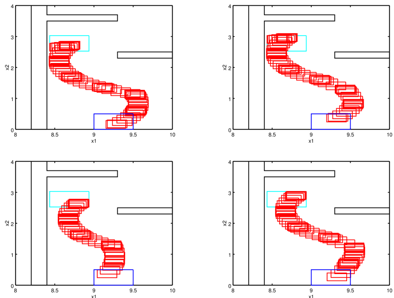
Figure 9: Example 5.4: Set simulation of the path planning example after bisection. The green boxes are the initial regions obtained by bisection, the blue box is the target region R_2 . The union of the red boxes is the reachability tube.
