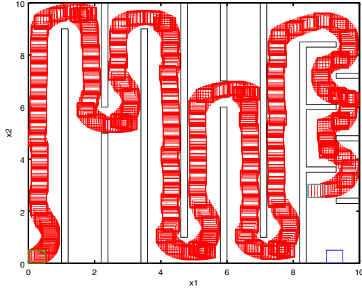
Figure 8: Example 5.4: Set simulation of the path planning example. The green box is the initial region R_1 , the blue box is the target region R_2 . The union of the red boxes is the reachability tube. In this case, the target region is not attained without bisection.
